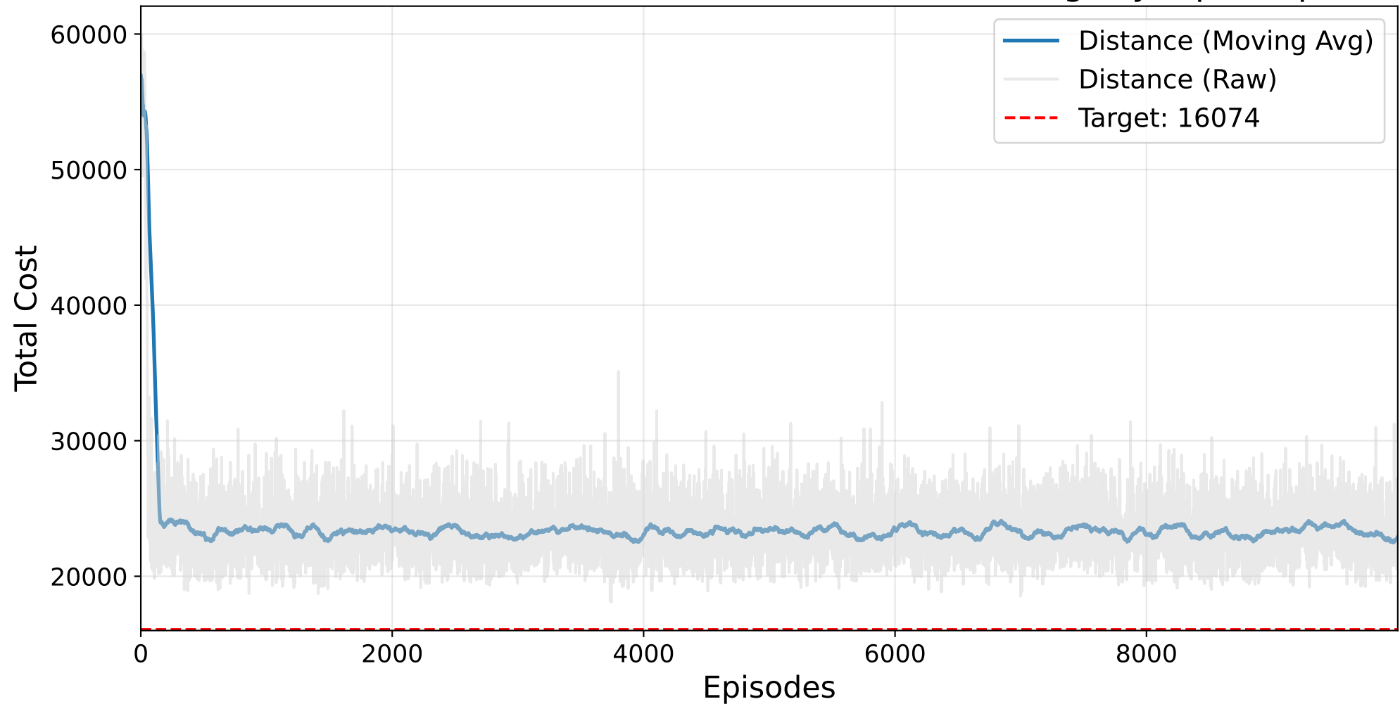
Final HYPERBAND TPE Masked AutoRL-SOP Training - ry48p.2.sop
